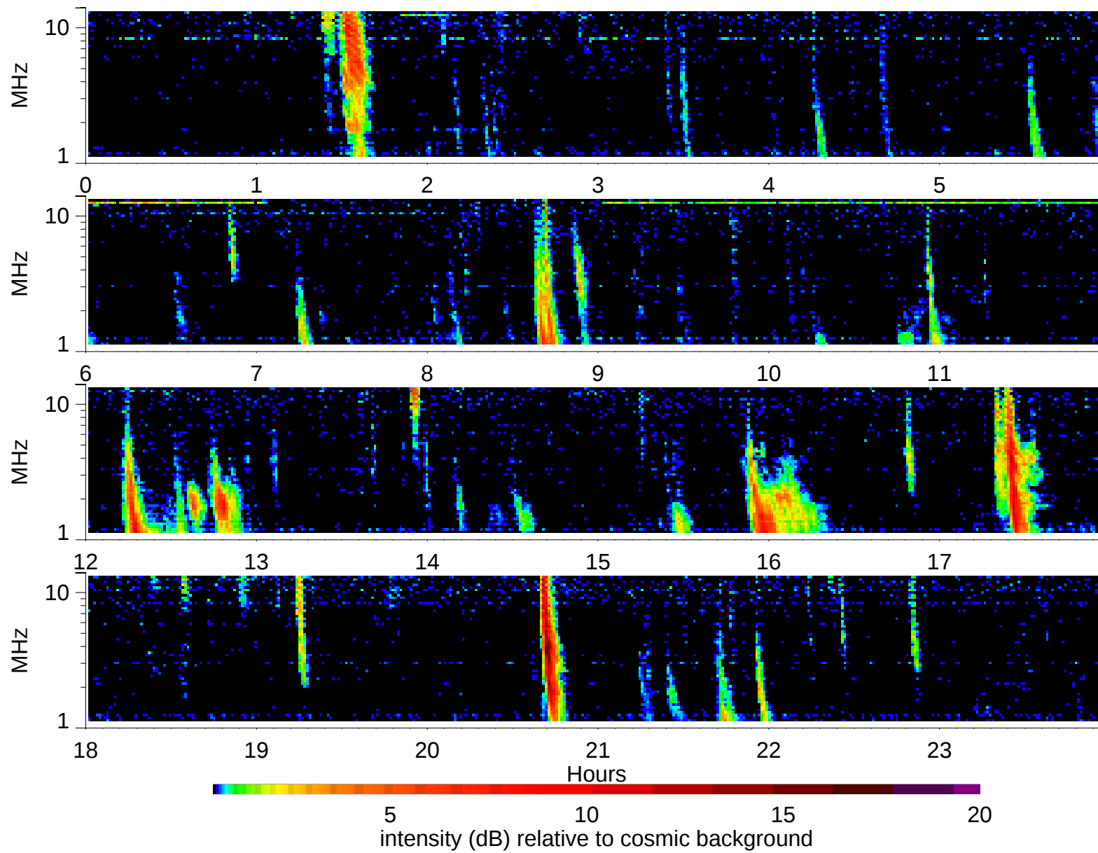
Wind Waves RAD2 receiver: 1998/11/18
