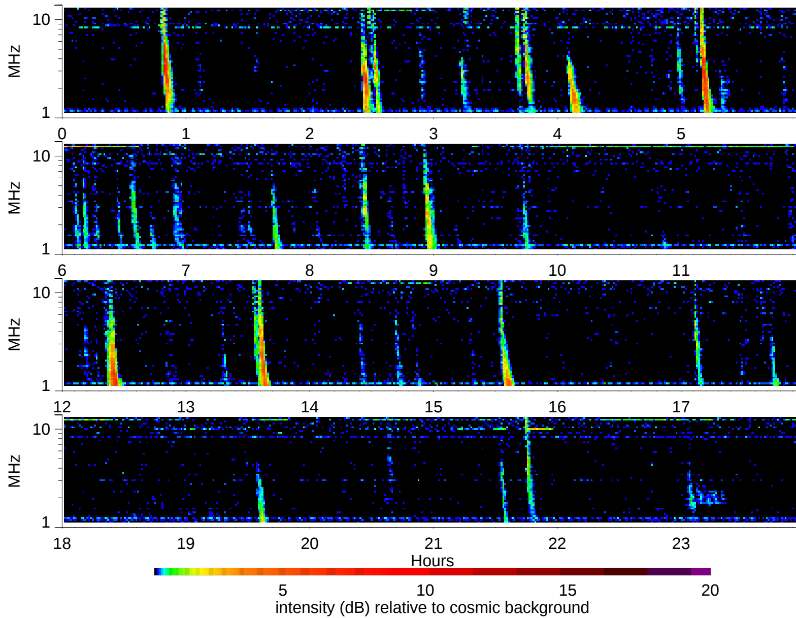
Wind Waves RAD2 receiver: 1998/11/19
