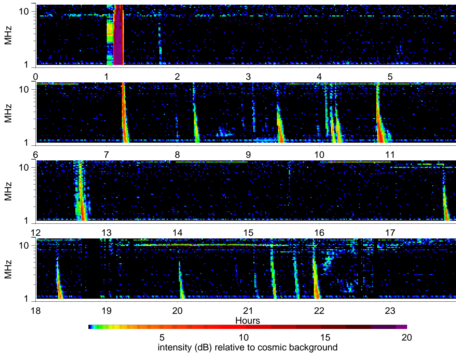
Wind Waves RAD2 receiver: 1998/11/20
