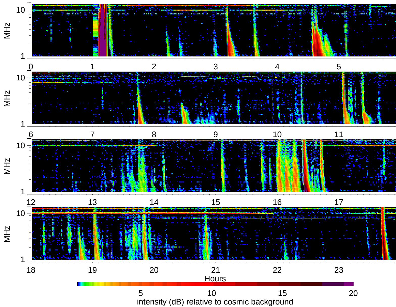
Wind Waves RAD2 receiver: 1998/12/6
