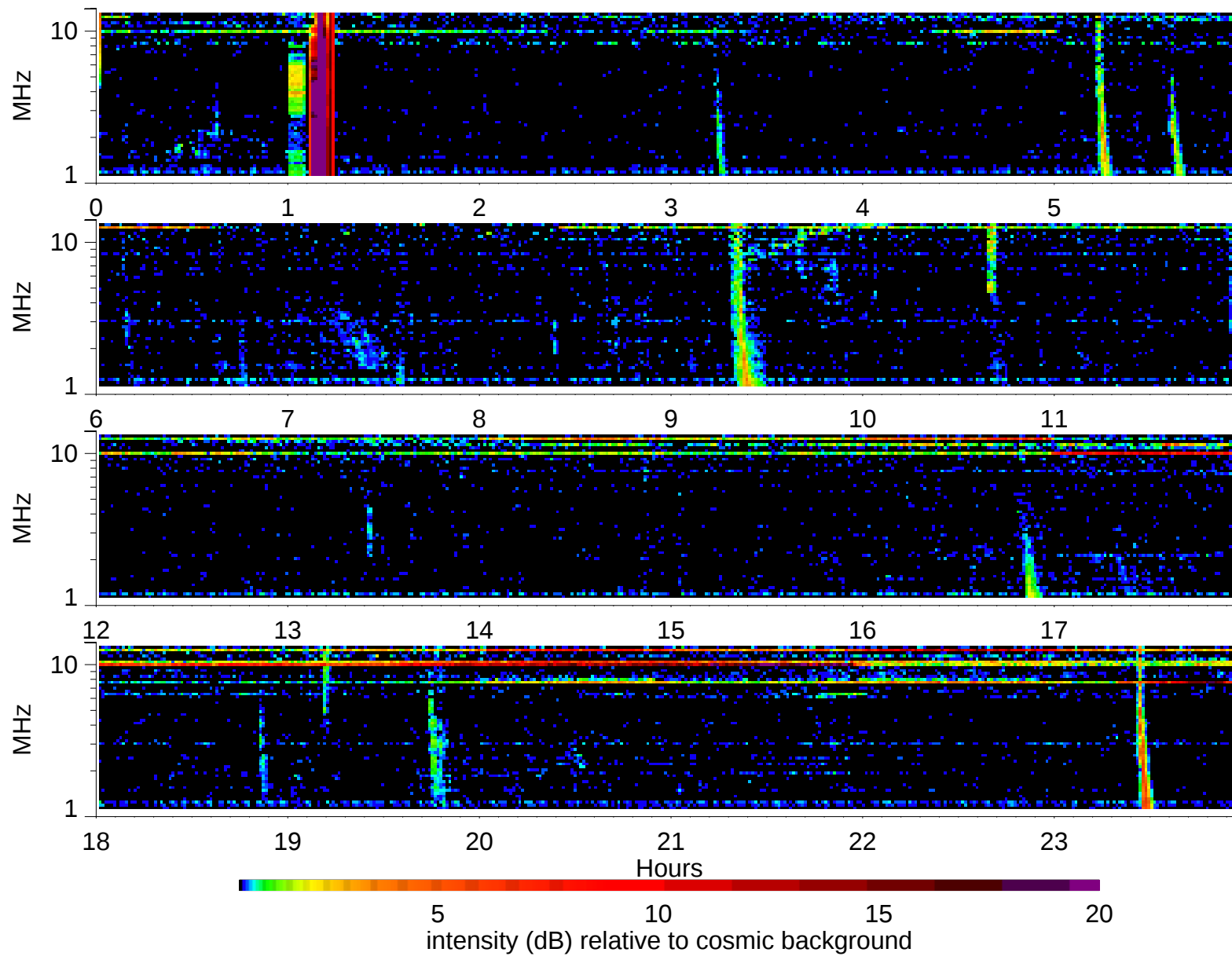
Wind Waves RAD2 receiver: 1998/12/10
