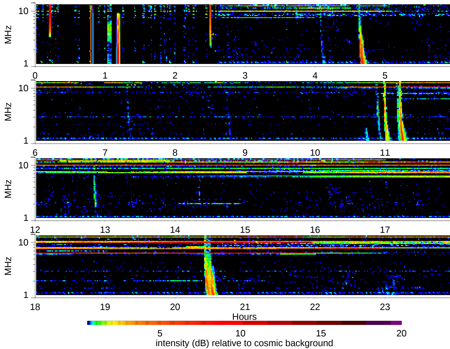
Wind Waves RAD2 receiver: 1998/12/12
