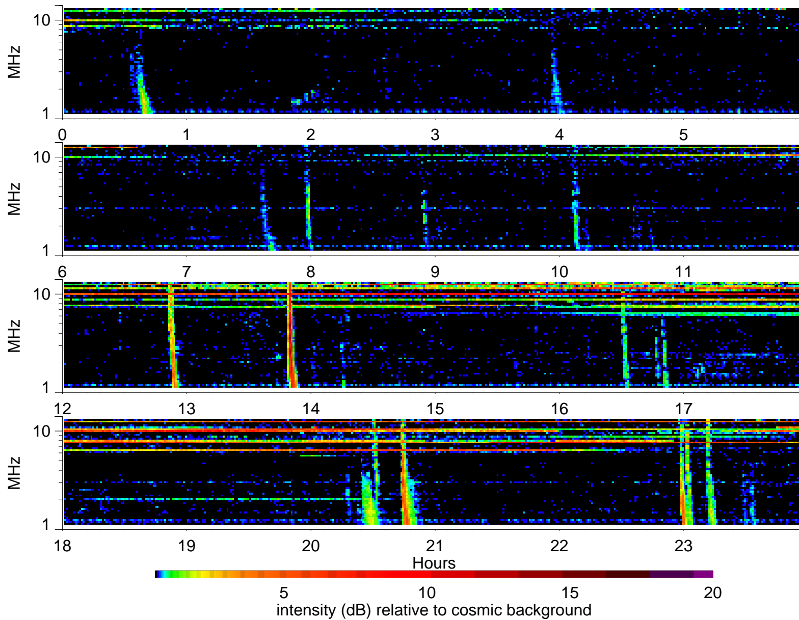
Wind Waves RAD2 receiver: 1998/12/13
