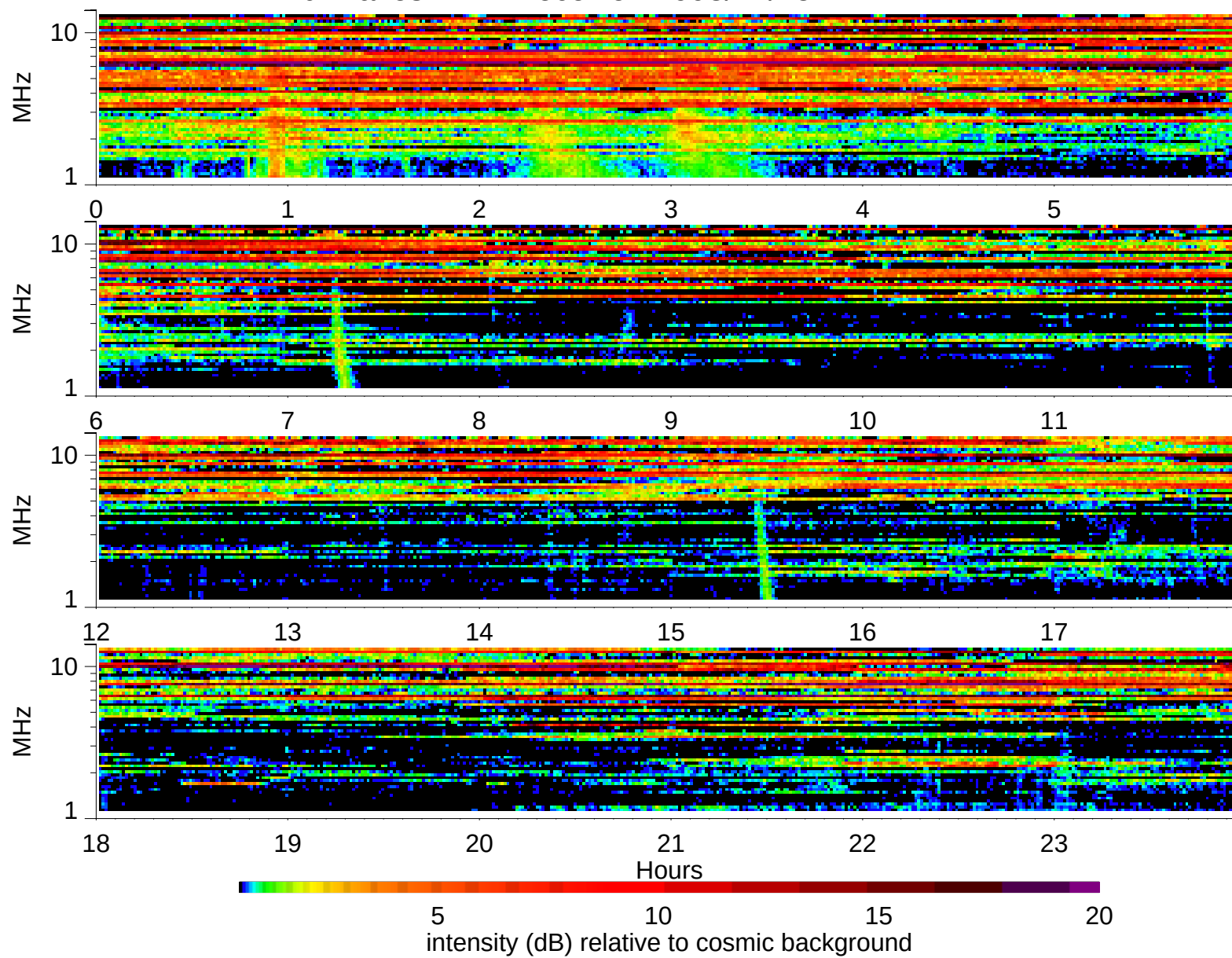
Wind Waves RAD2 receiver: 1998/12/15
