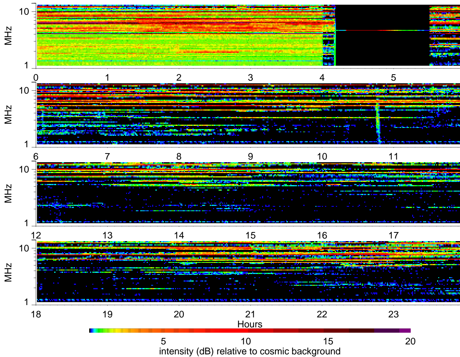
Wind Waves RAD2 receiver: 1998/12/16
