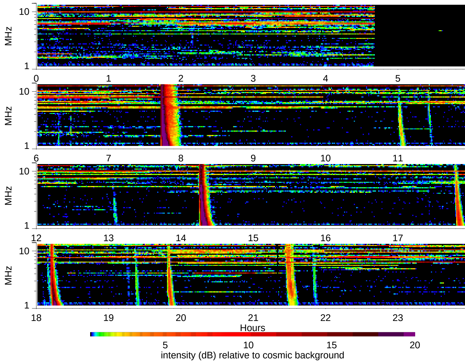
Wind Waves RAD2 receiver: 1998/12/17
