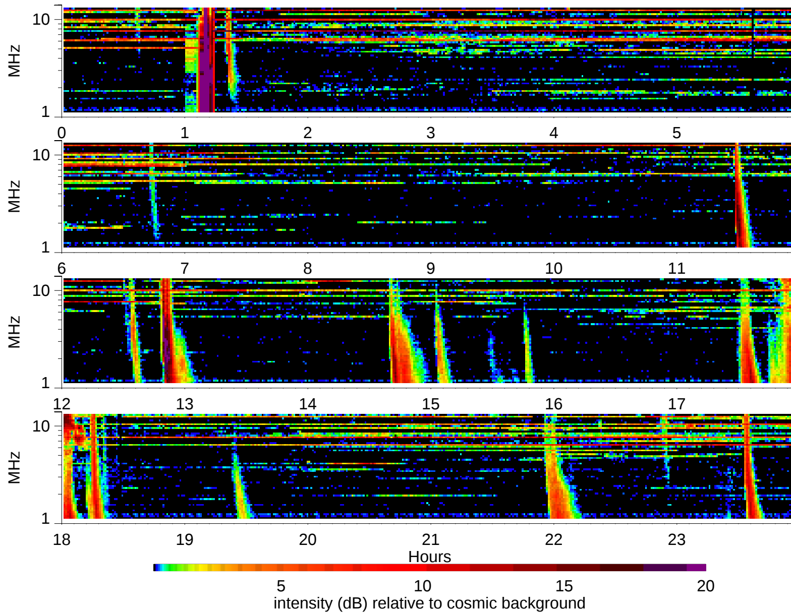
Wind Waves RAD2 receiver: 1998/12/18
