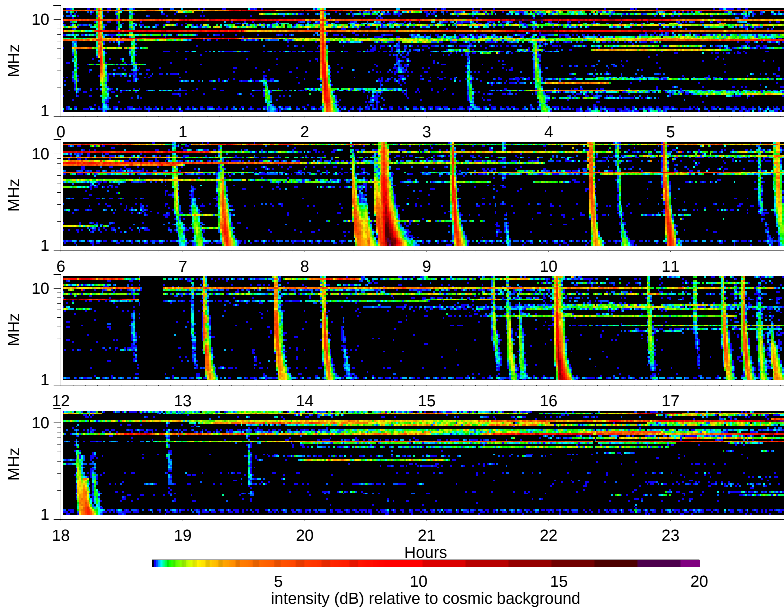
Wind Waves RAD2 receiver: 1998/12/19
