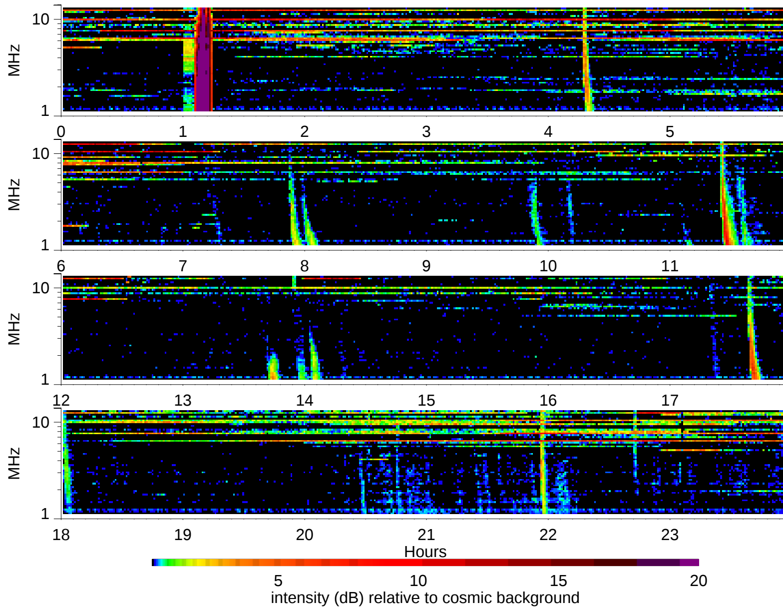
Wind Waves RAD2 receiver: 1998/12/20
