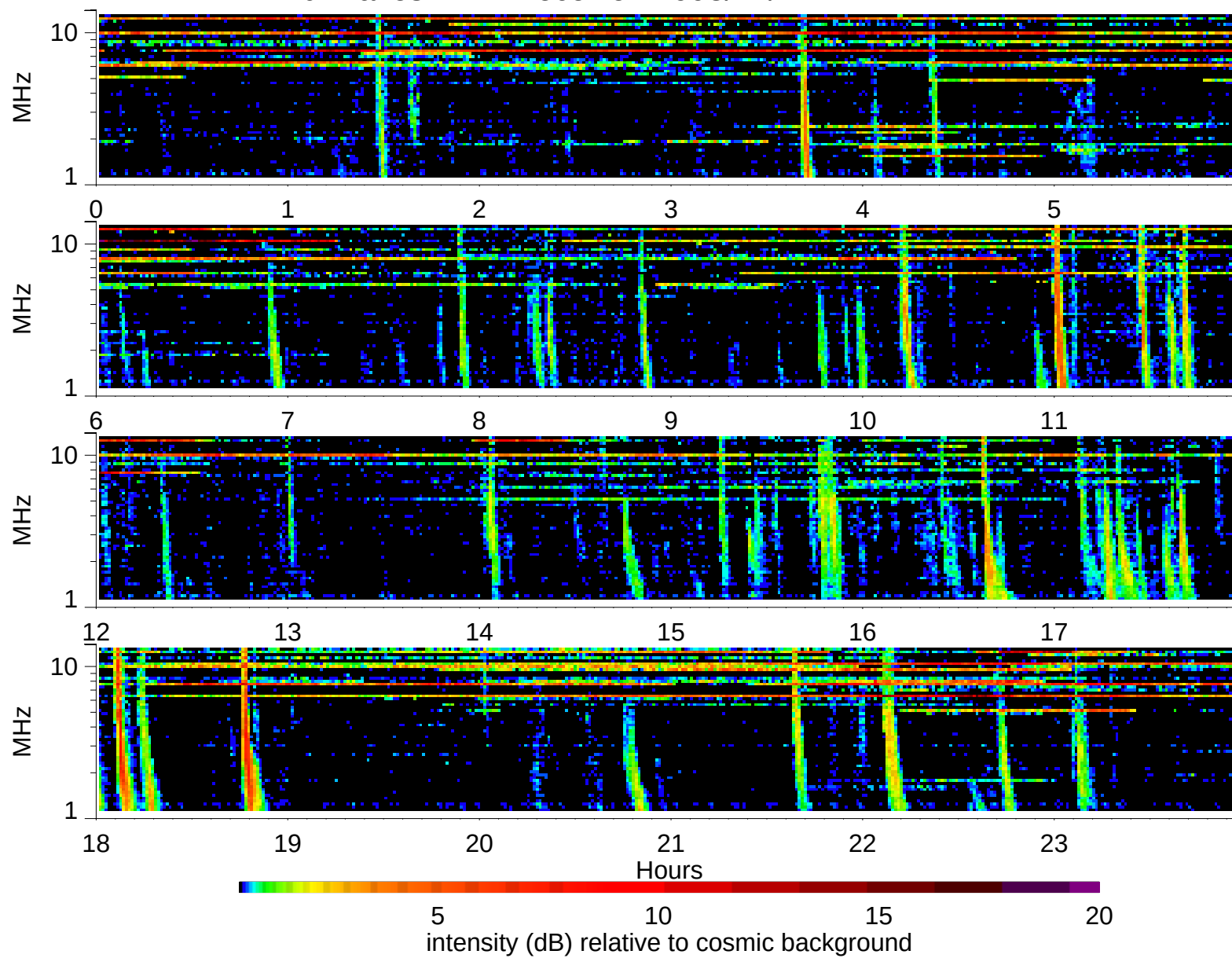
Wind Waves RAD2 receiver: 1998/12/21
