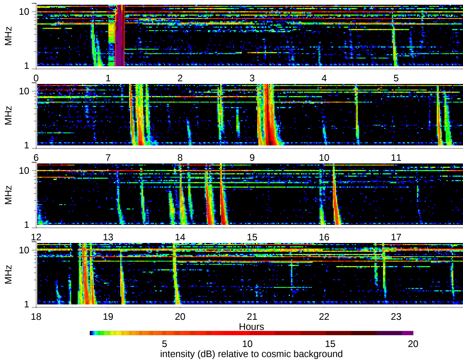
Wind Waves RAD2 receiver: 1998/12/22
