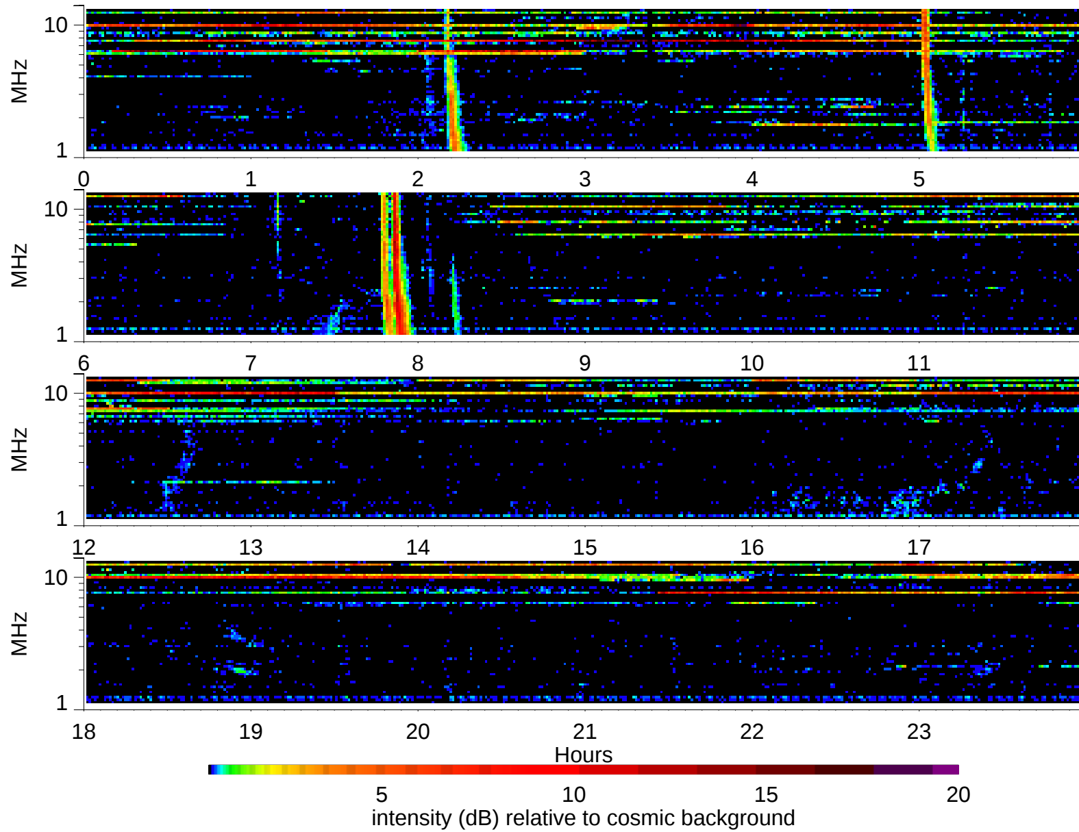
Wind Waves RAD2 receiver: 1998/12/25
