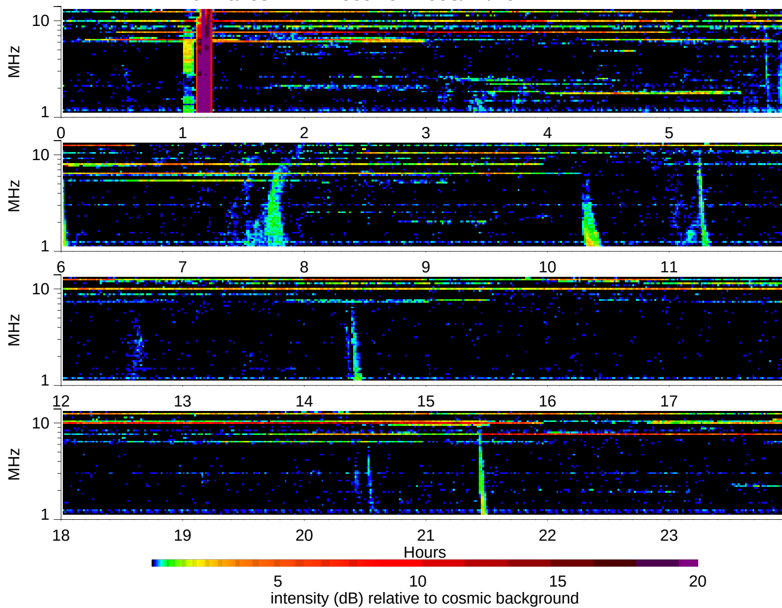
Wind Waves RAD2 receiver: 1998/12/26
