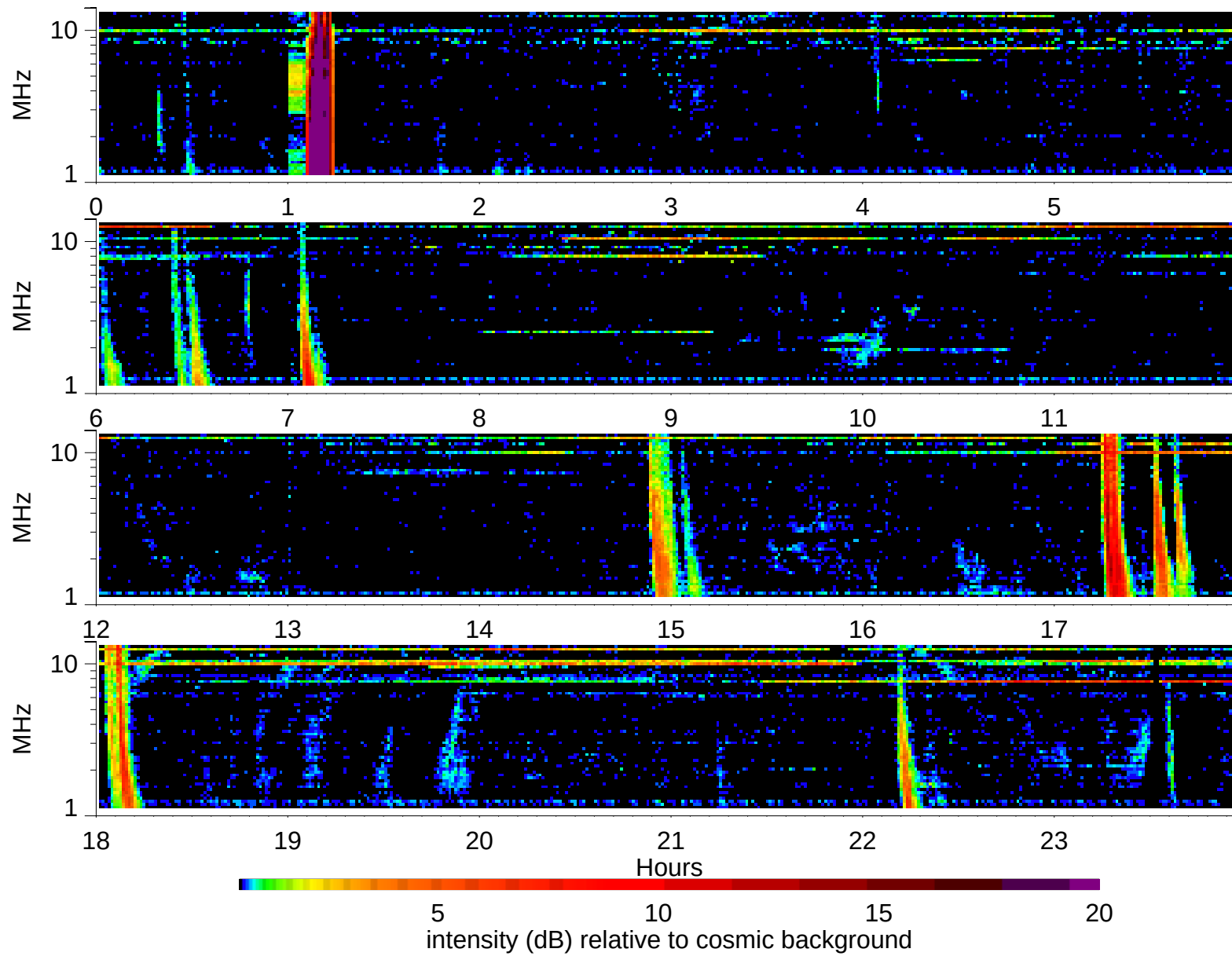
Wind Waves RAD2 receiver: 1998/12/28
