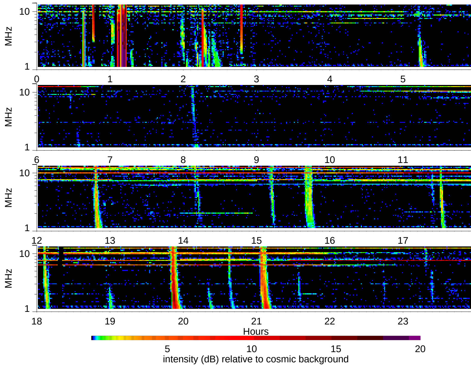
Wind Waves RAD2 receiver: 1998/12/30
