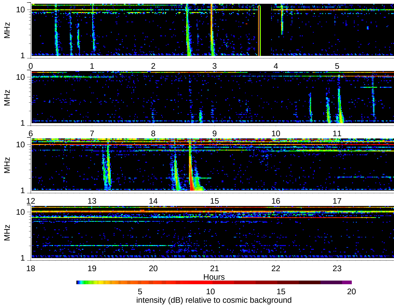
Wind Waves RAD2 receiver: 1998/12/31
