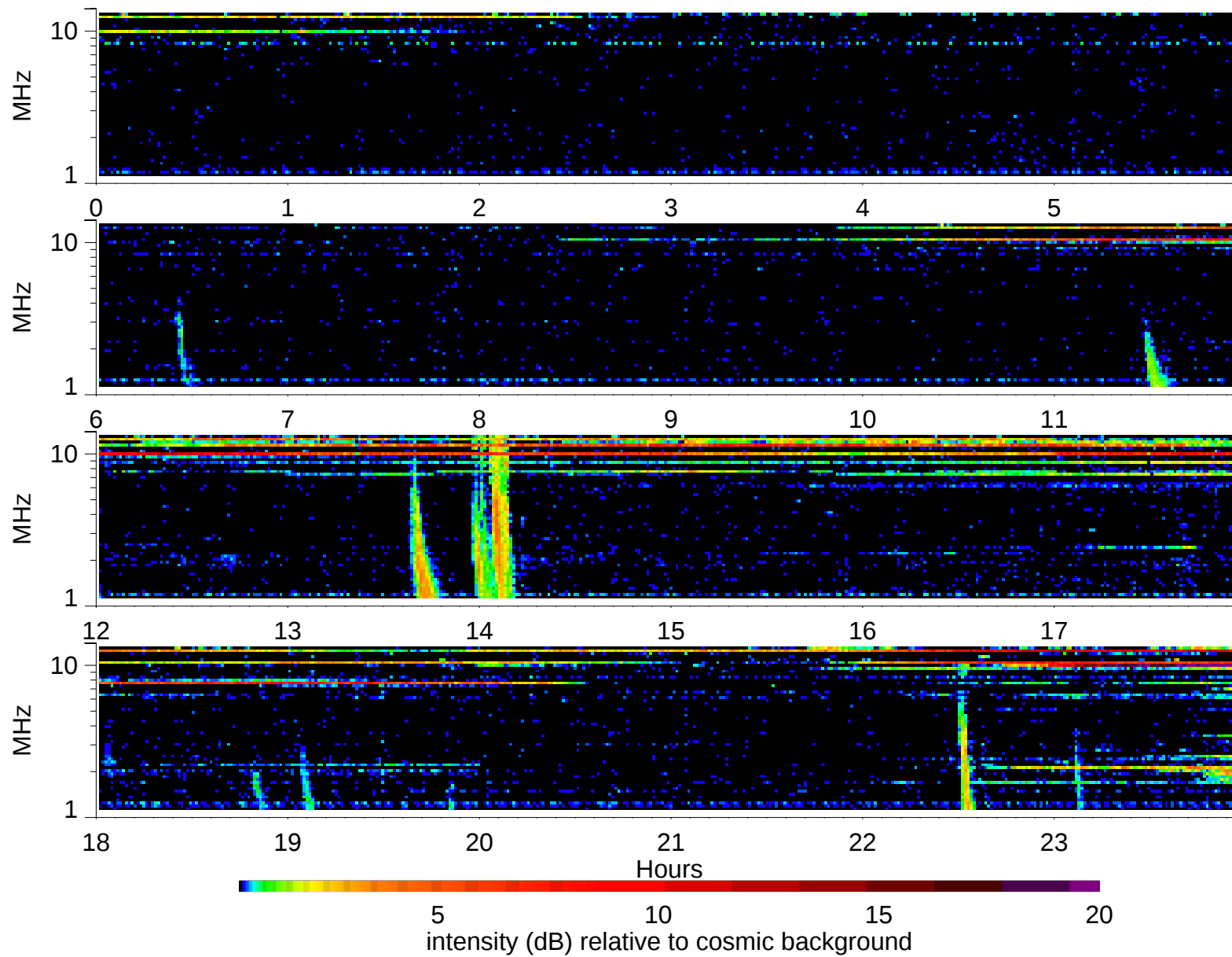
Wind Waves RAD2 receiver: 1999/1/1
