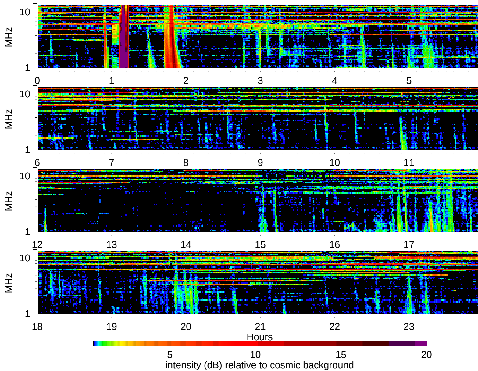
Wind Waves RAD2 receiver: 1999/1/6
