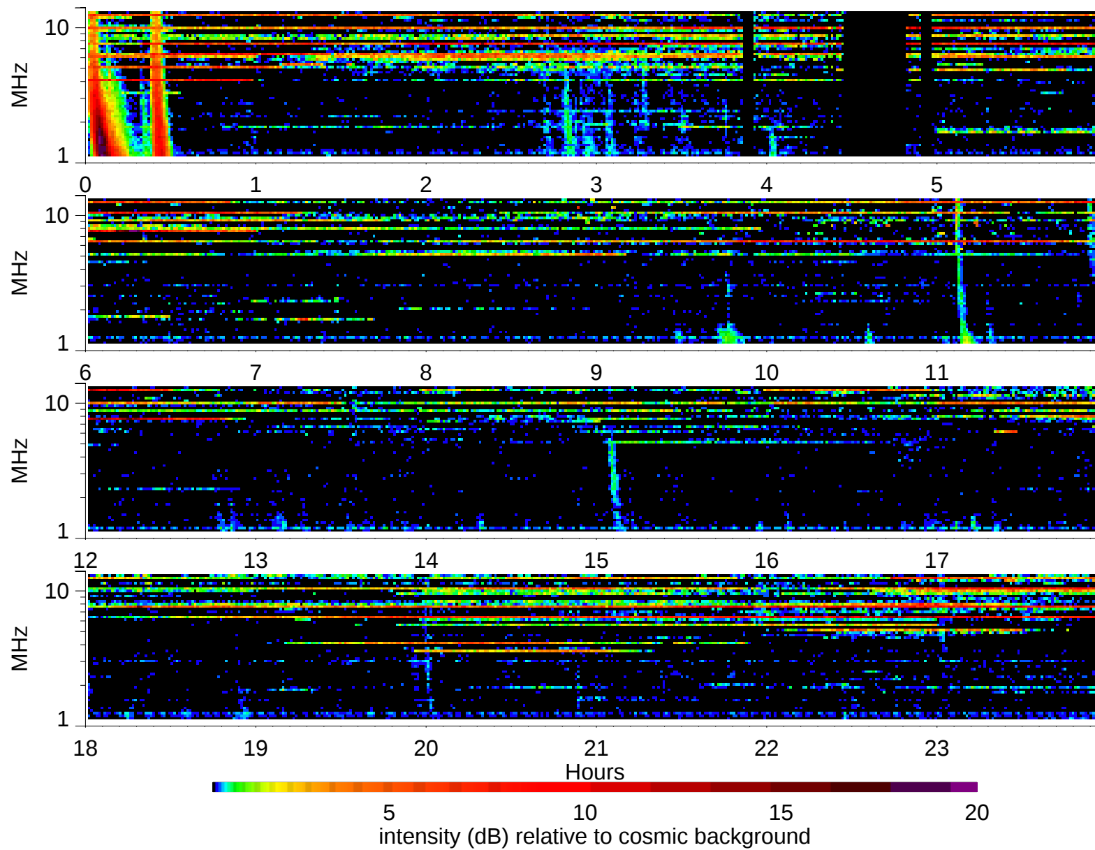
Wind Waves RAD2 receiver: 1999/1/7
