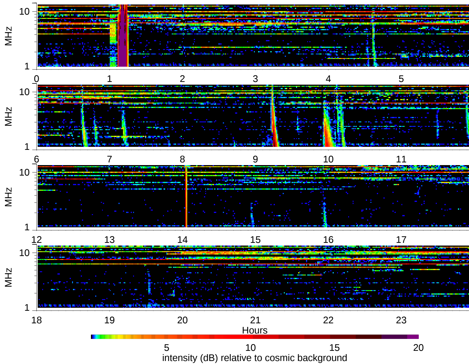
Wind Waves RAD2 receiver: 1999/1/8
