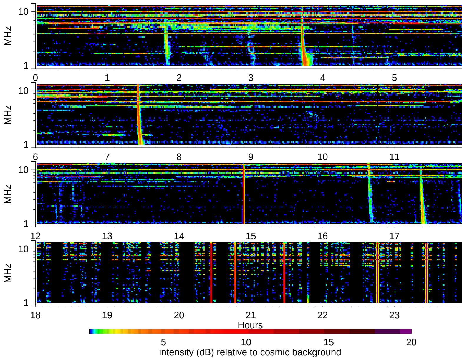
Wind Waves RAD2 receiver: 1999/1/9
