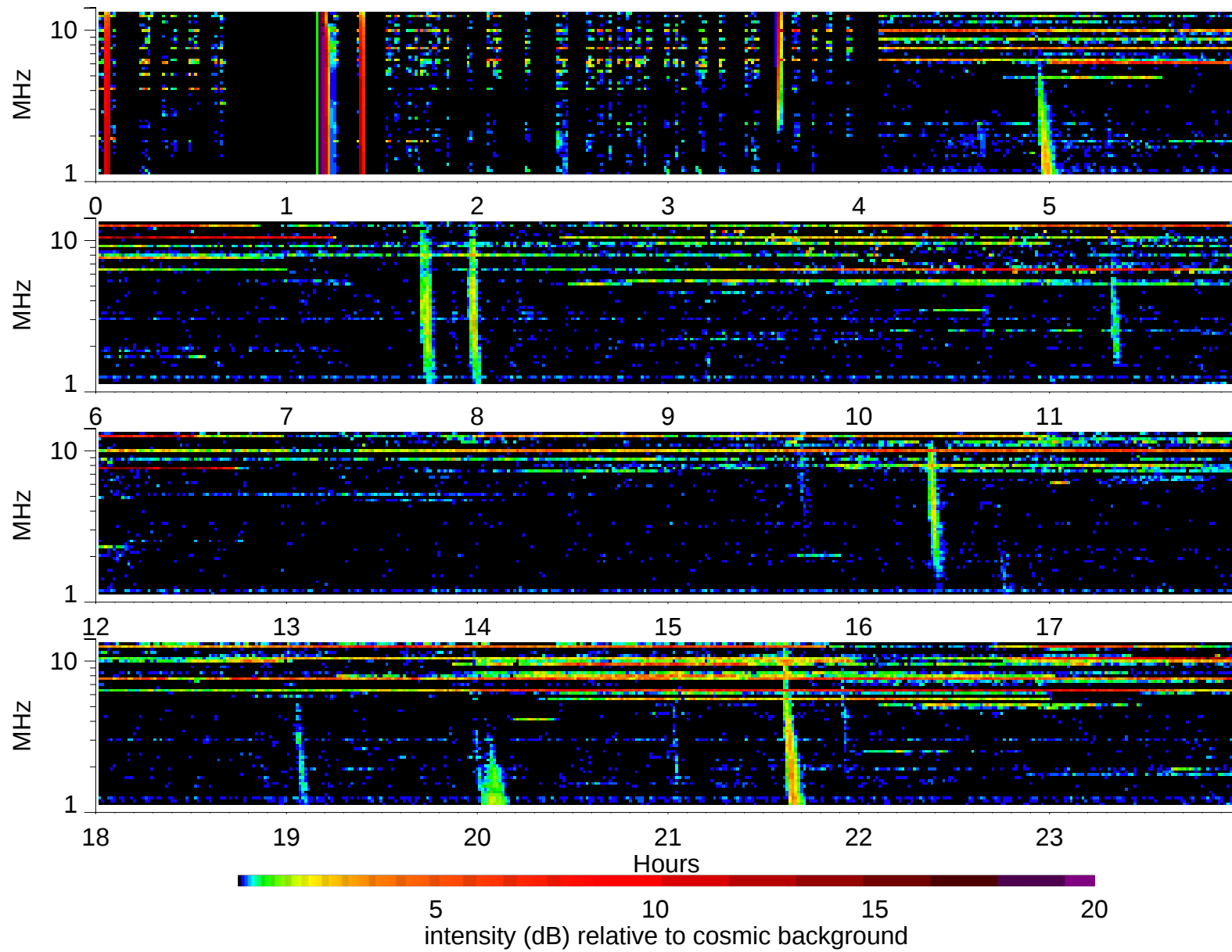
Wind Waves RAD2 receiver: 1999/1/10
