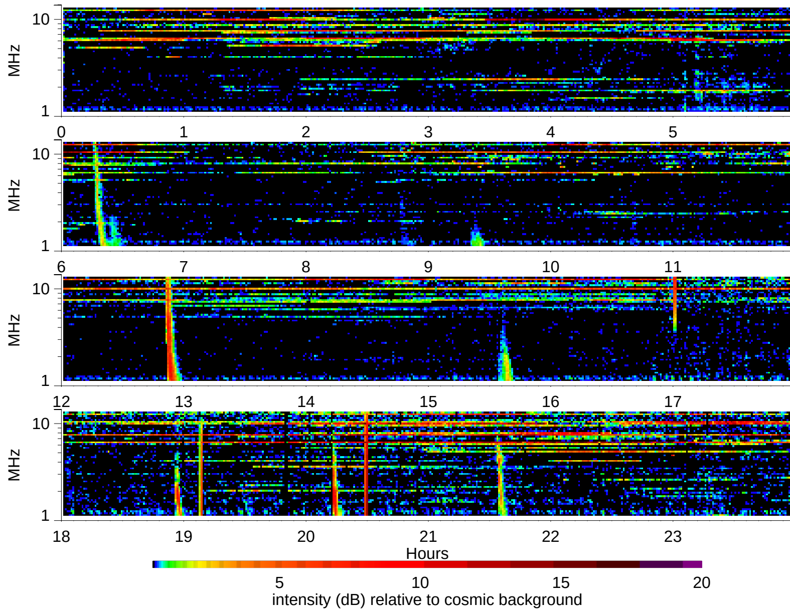
Wind Waves RAD2 receiver: 1999/1/13
