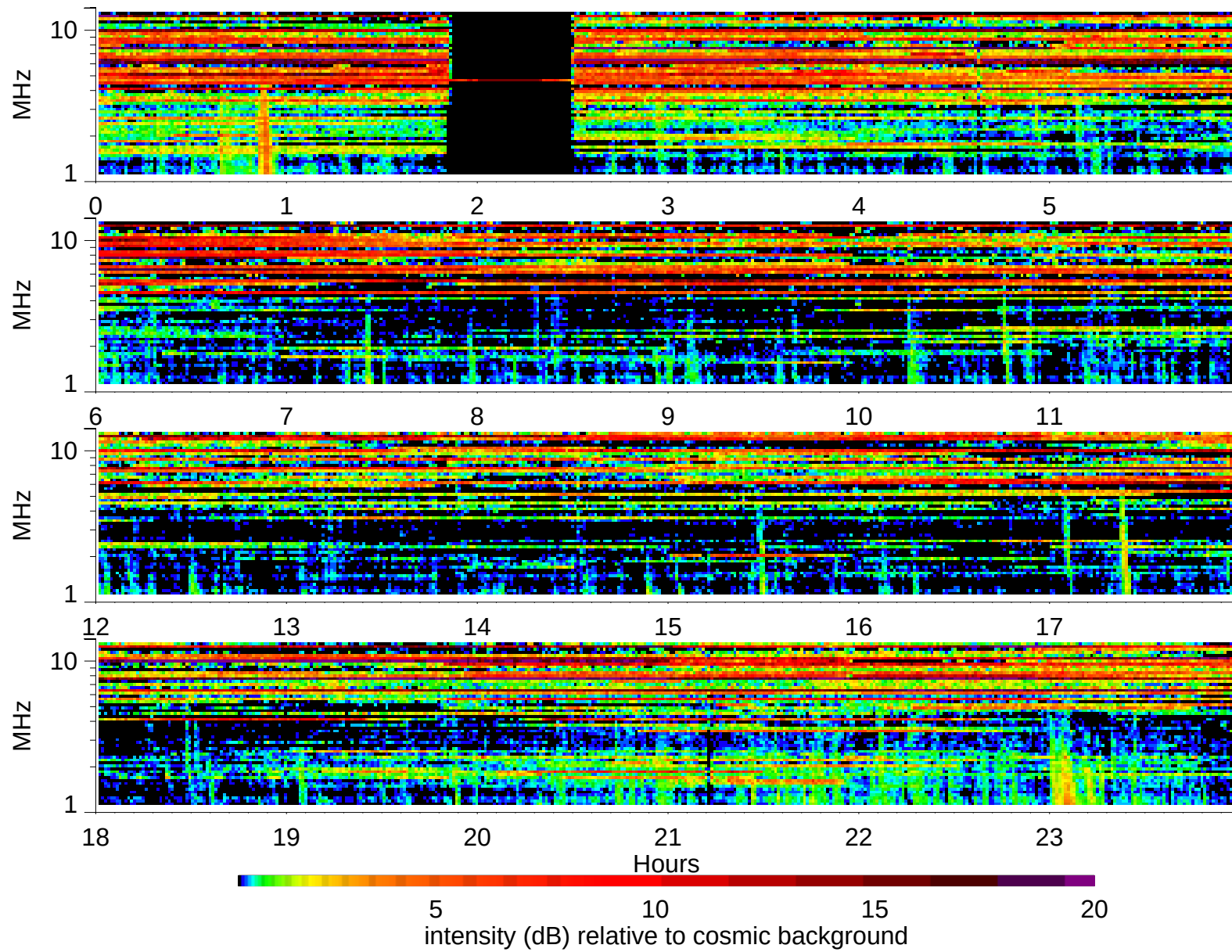
Wind Waves RAD2 receiver: 1999/1/19
