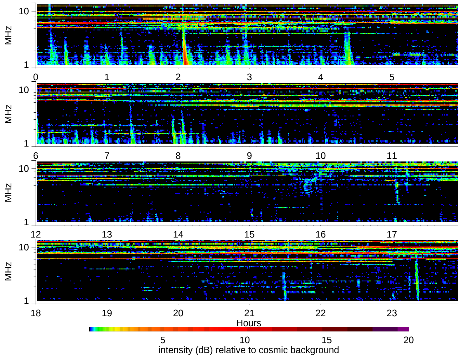
Wind Waves RAD2 receiver: 1999/1/23
