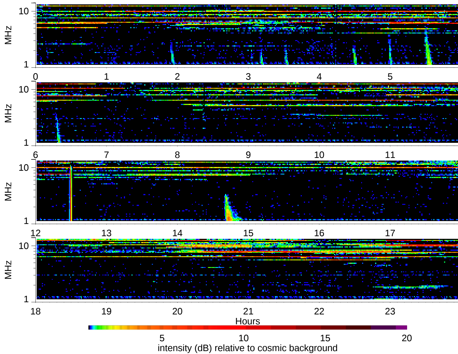
Wind Waves RAD2 receiver: 1999/1/29
