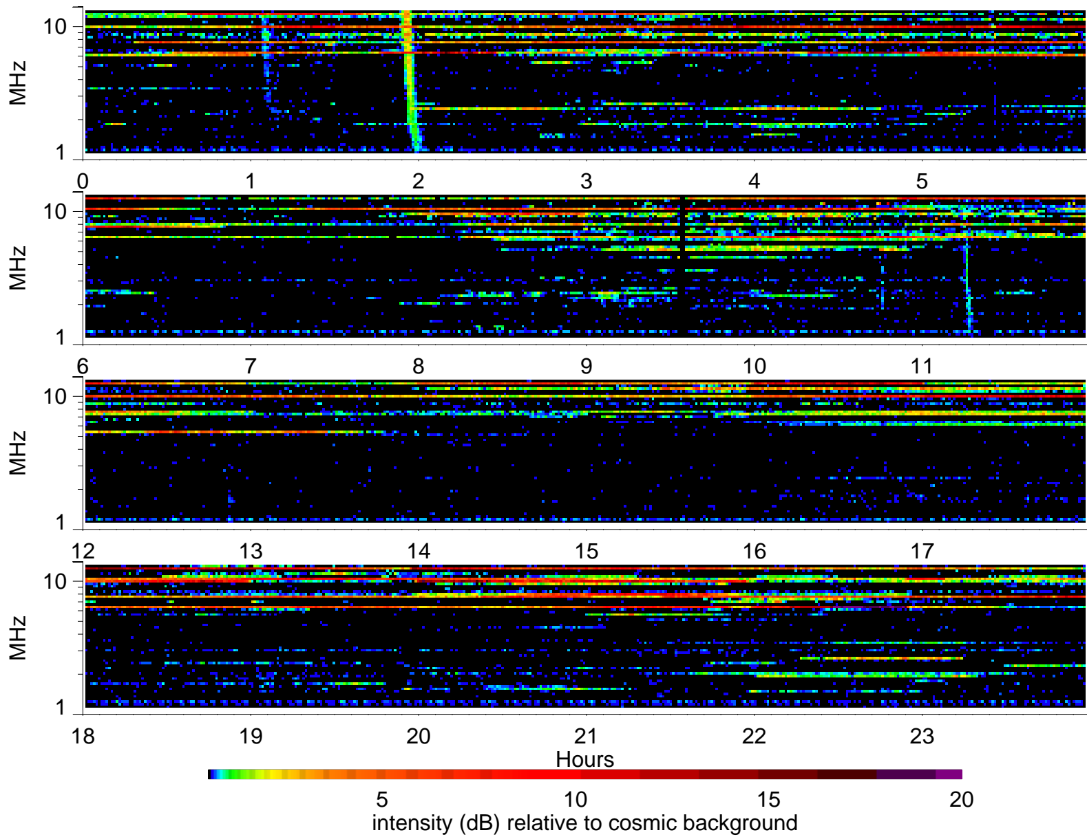
Wind Waves RAD2 receiver: 1999/2/2
