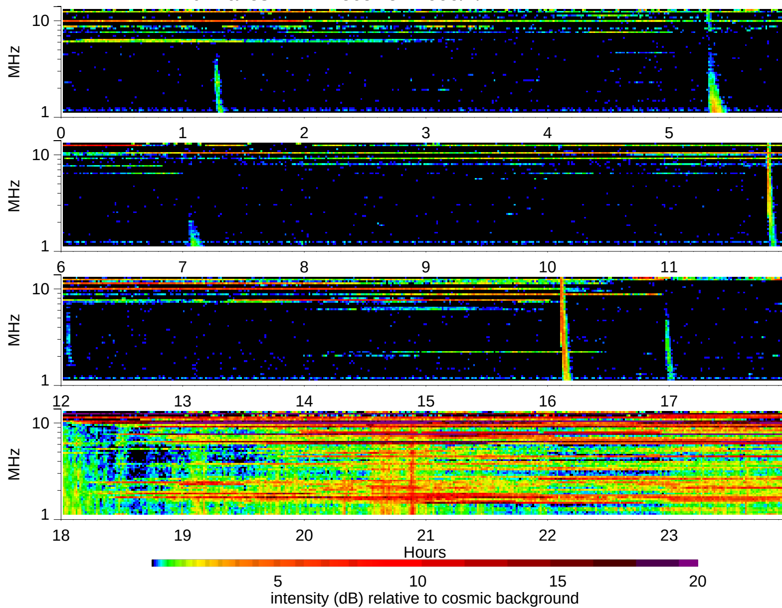
Wind Waves RAD2 receiver: 1999/2/4
