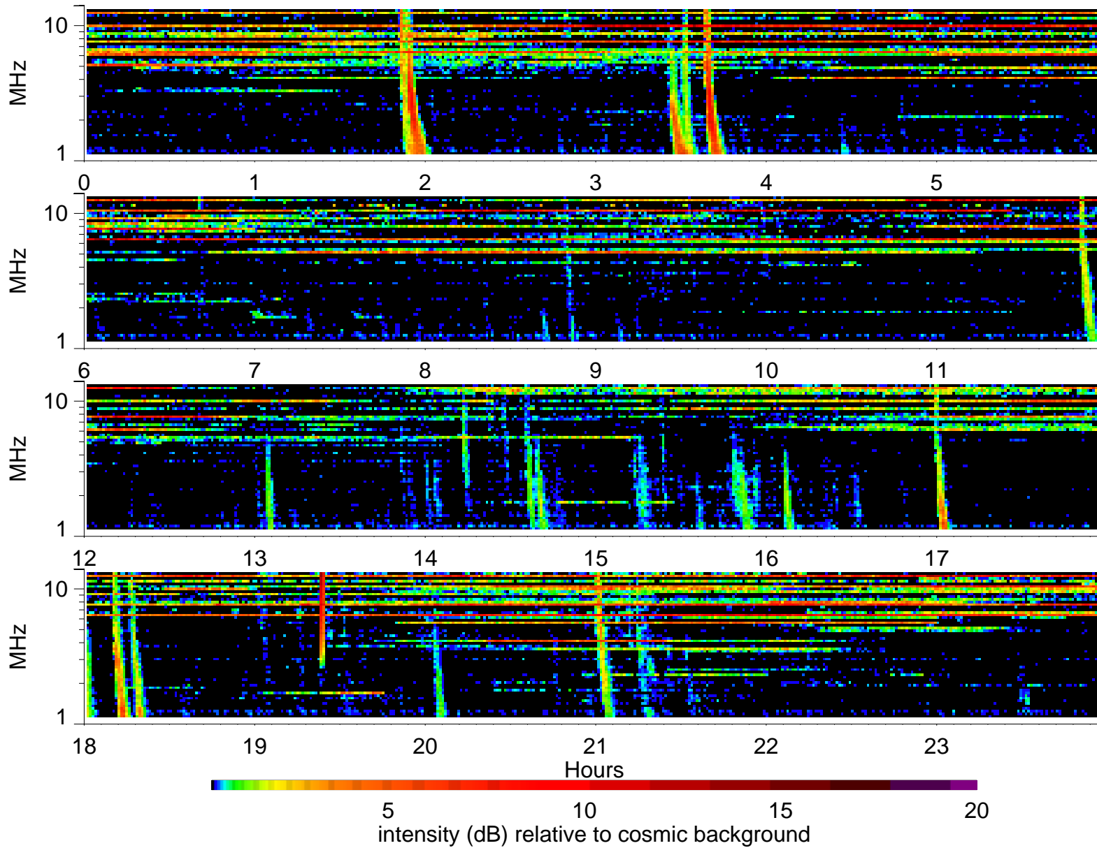
Wind Waves RAD2 receiver: 1999/2/10
