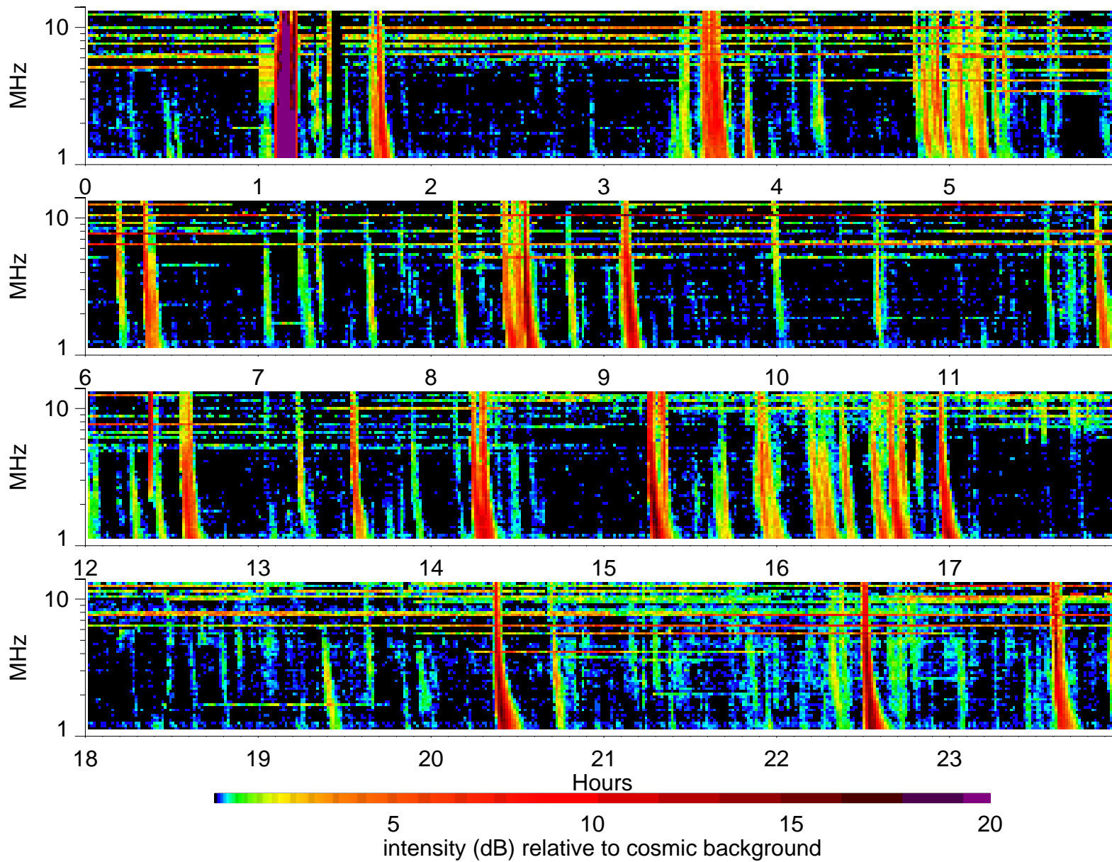
Wind Waves RAD2 receiver: 1999/2/13
