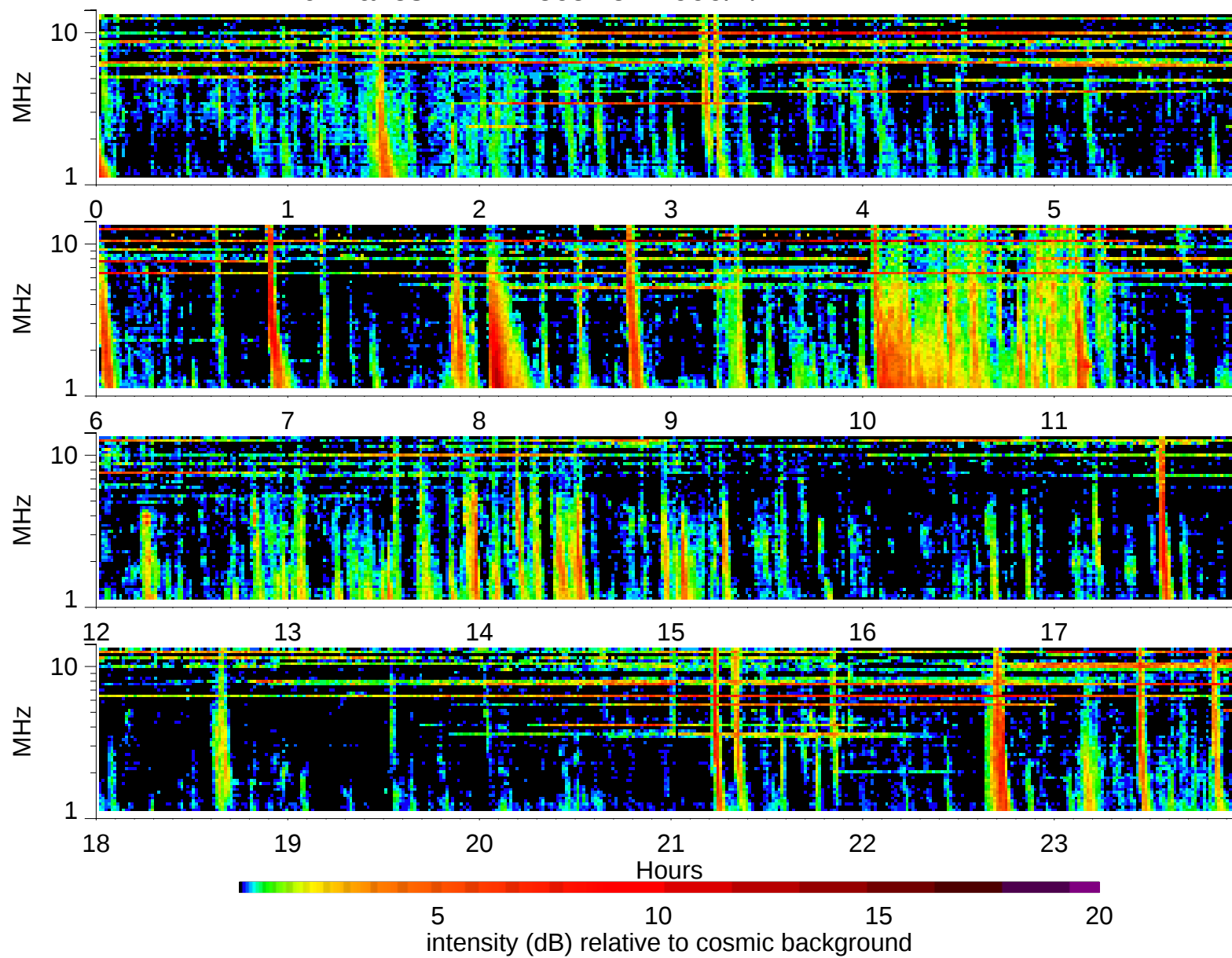
Wind Waves RAD2 receiver: 1999/2/14
