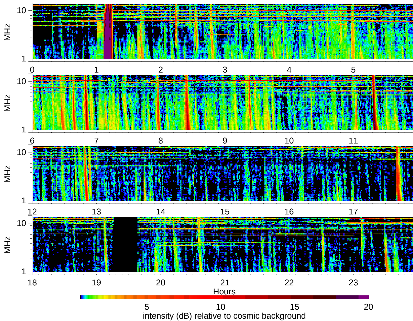
Wind Waves RAD2 receiver: 1999/2/15
