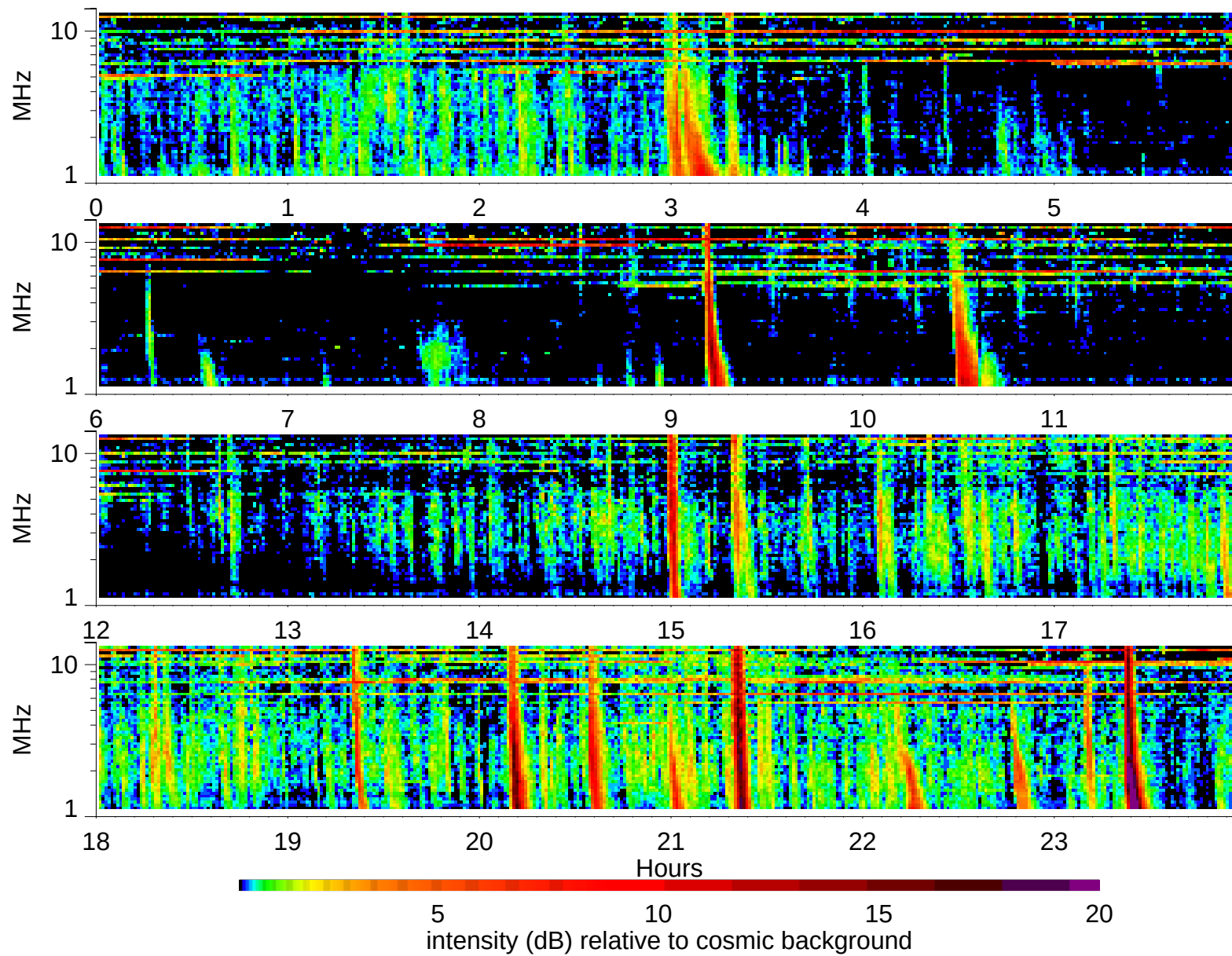
Wind Waves RAD2 receiver: 1999/2/16
