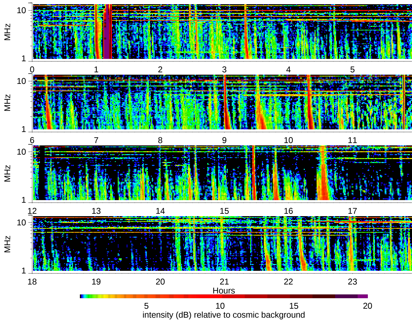
Wind Waves RAD2 receiver: 1999/2/17
