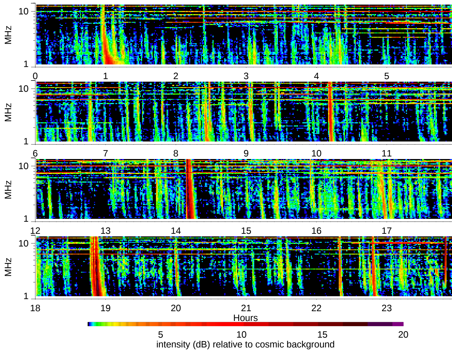
Wind Waves RAD2 receiver: 1999/2/18
