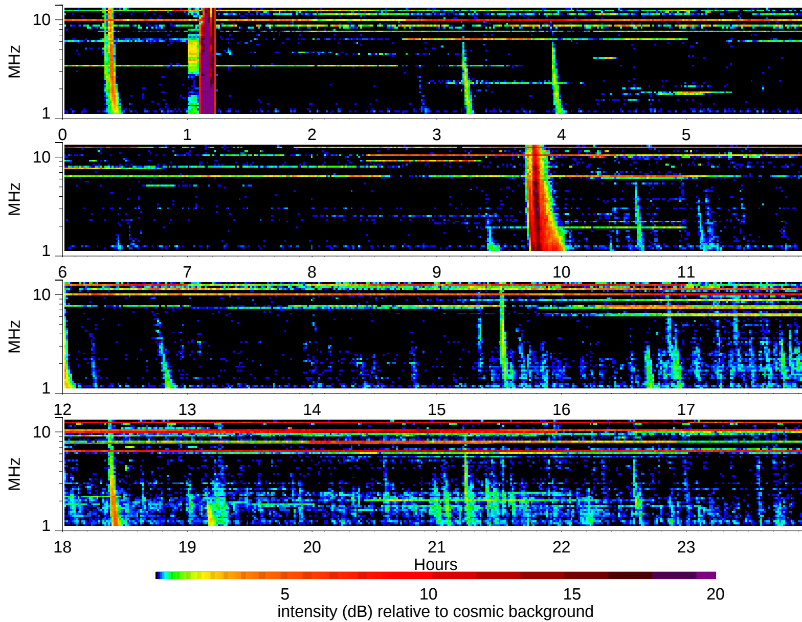
Wind Waves RAD2 receiver: 1999/2/21
