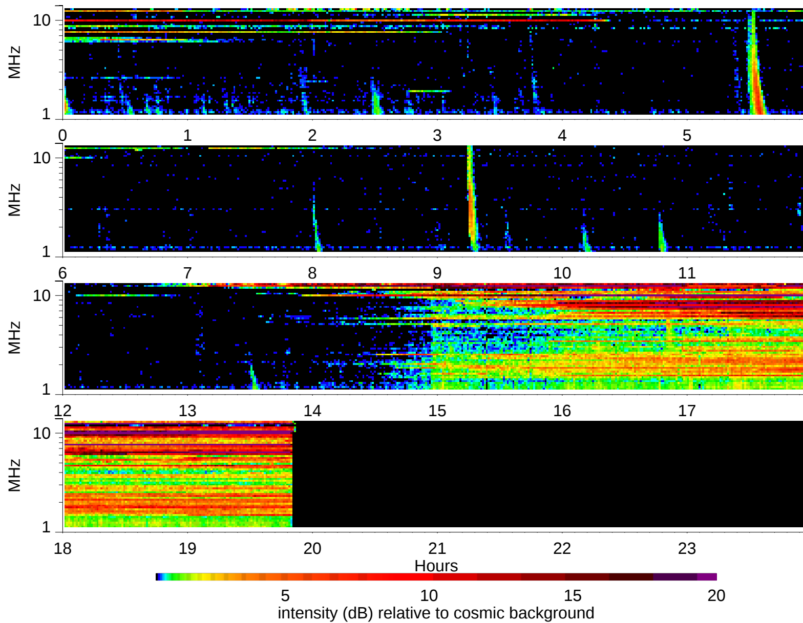
Wind Waves RAD2 receiver: 1999/2/22
