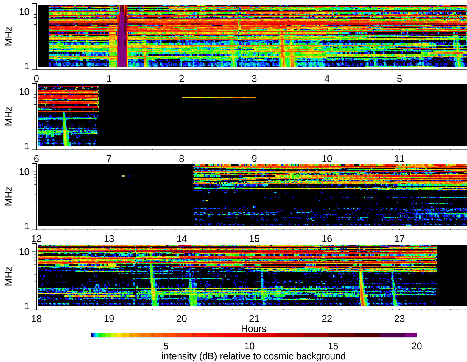
Wind Waves RAD2 receiver: 1999/2/23
