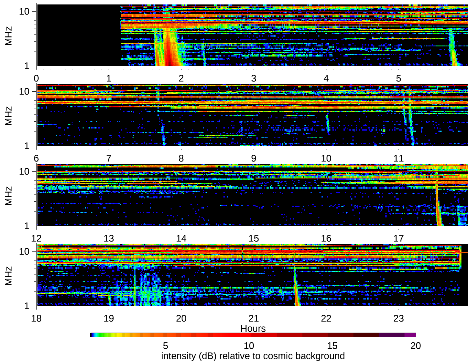
Wind Waves RAD2 receiver: 1999/2/24
