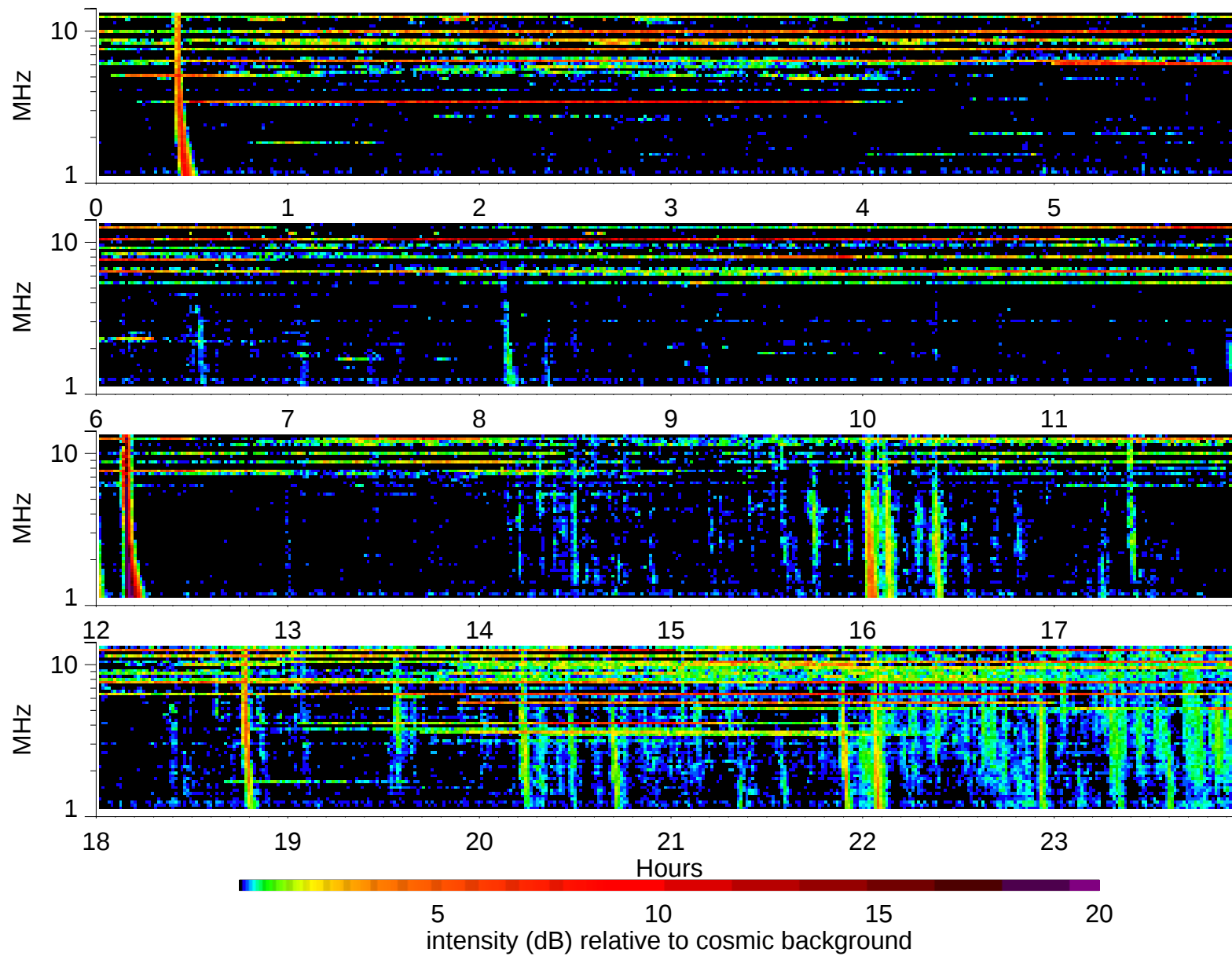
Wind Waves RAD2 receiver: 1999/3/2
