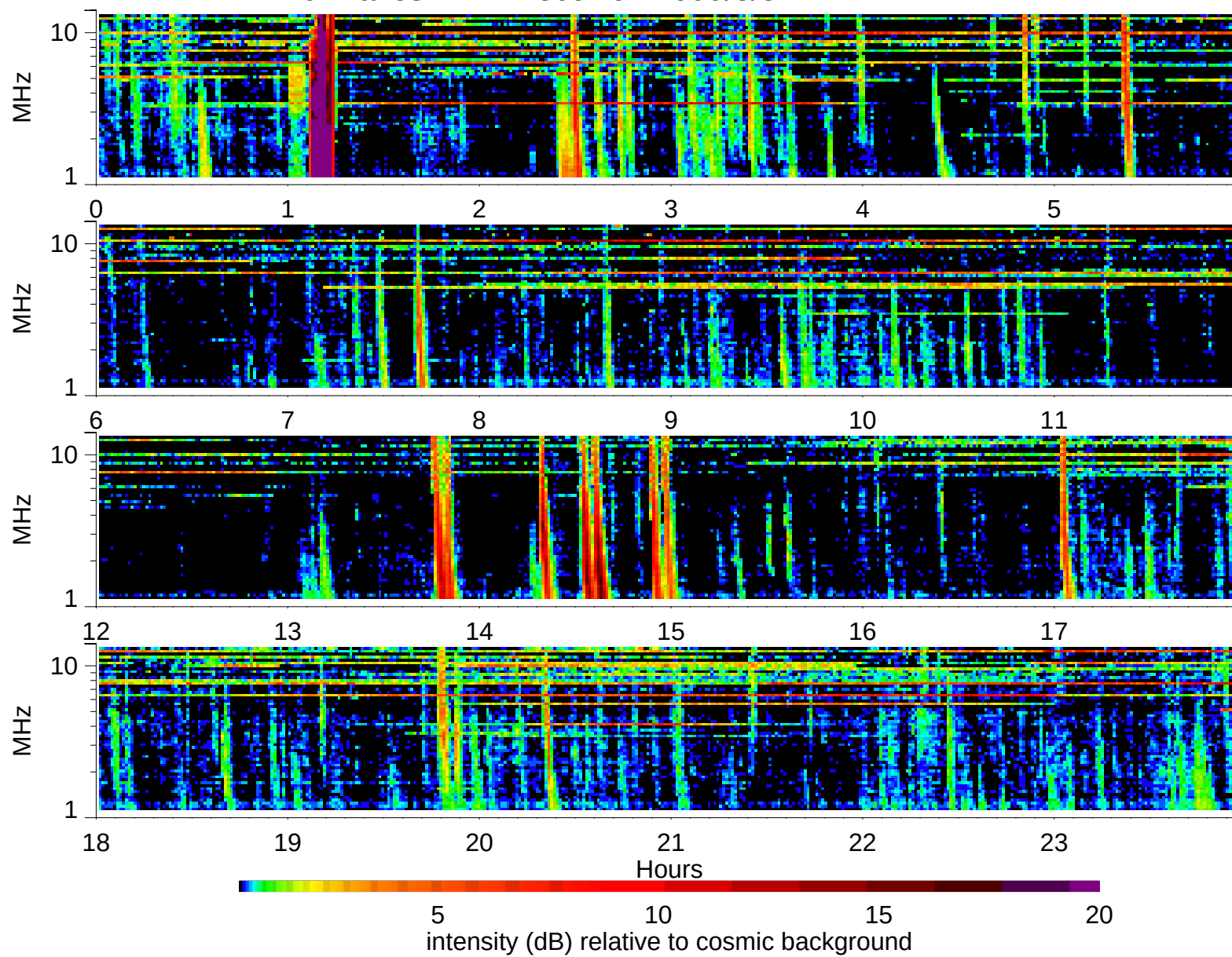
Wind Waves RAD2 receiver: 1999/3/3
