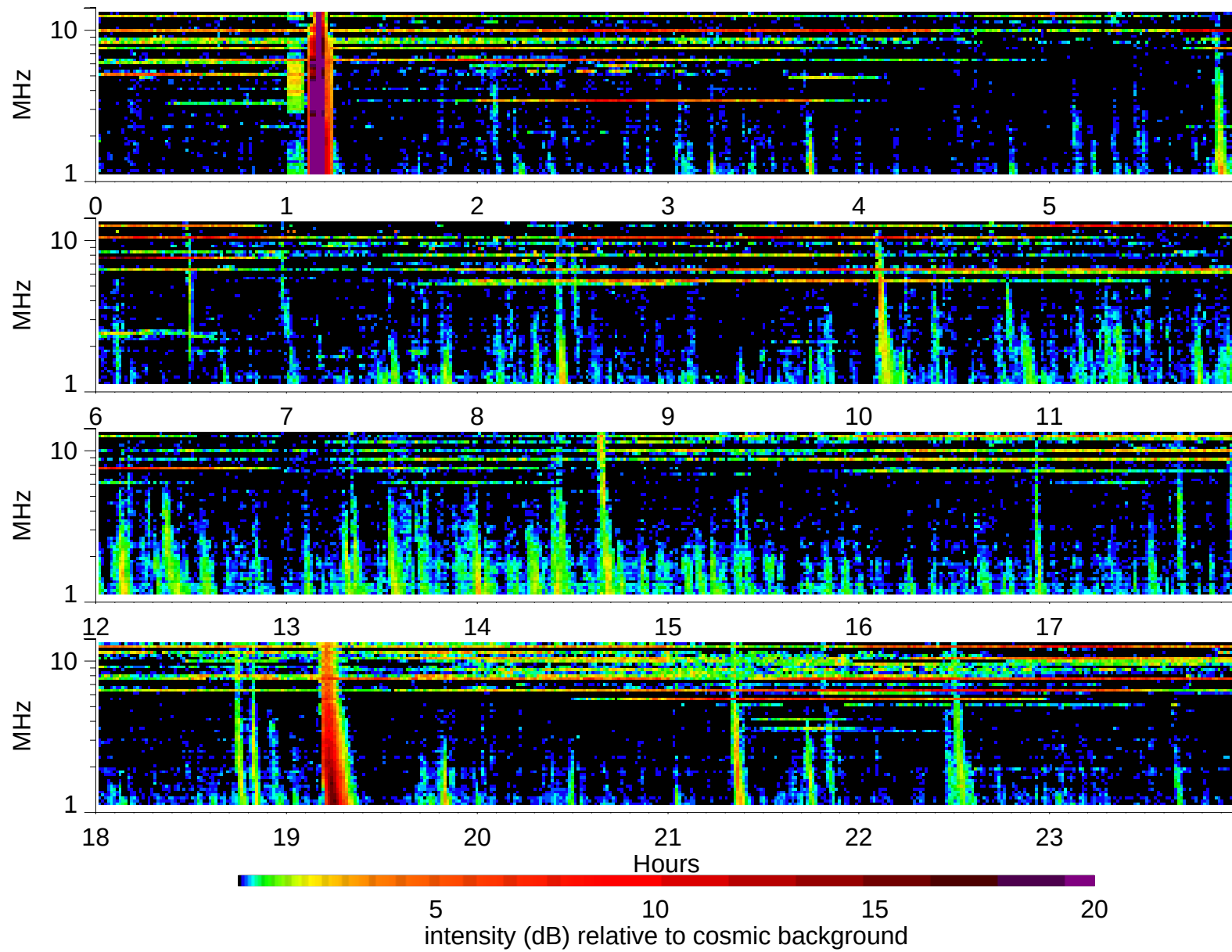
Wind Waves RAD2 receiver: 1999/3/5
