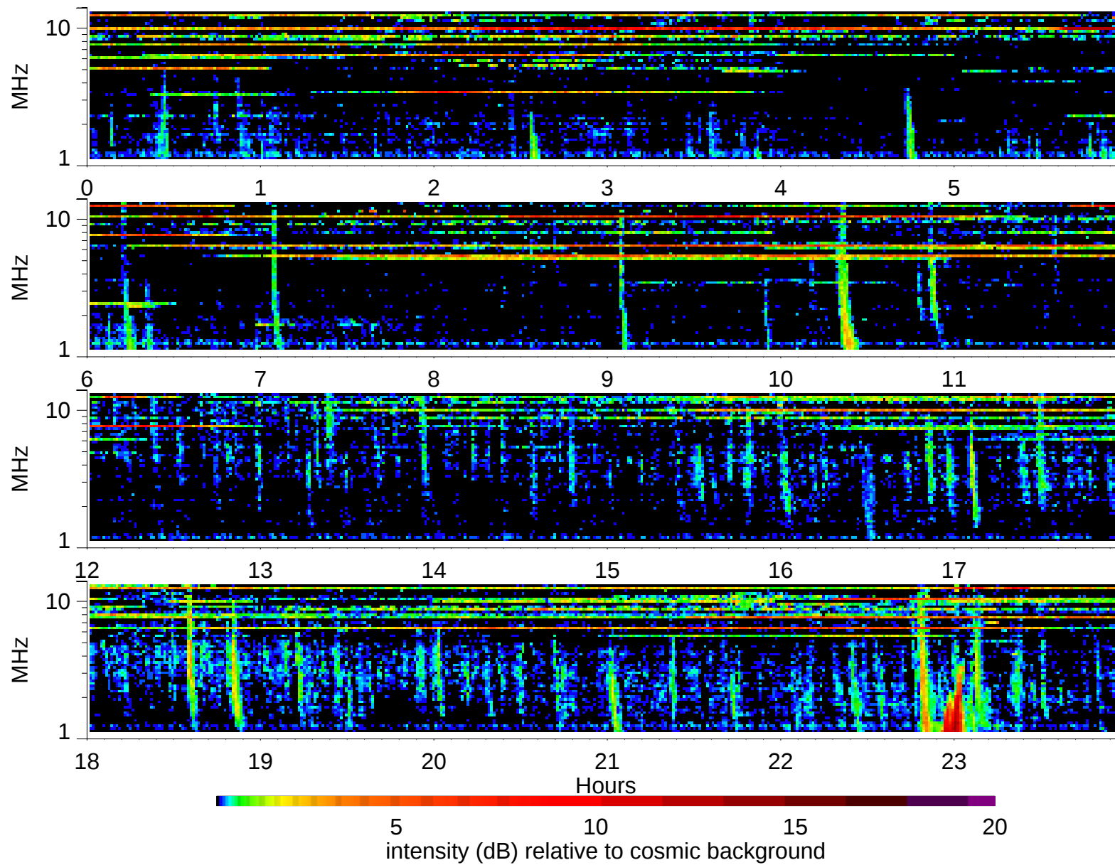
Wind Waves RAD2 receiver: 1999/3/6
