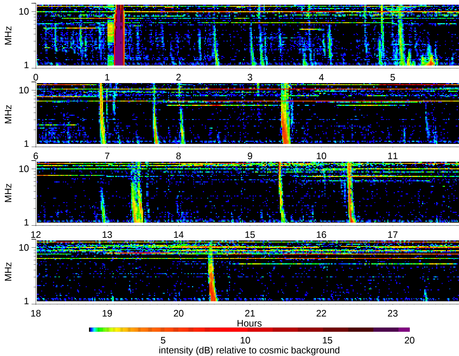
Wind Waves RAD2 receiver: 1999/3/7
