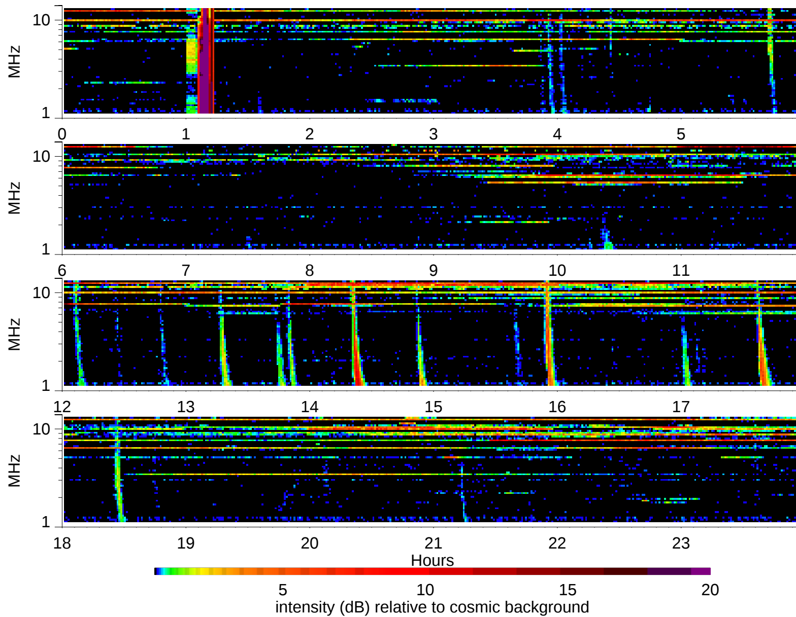
Wind Waves RAD2 receiver: 1999/3/9
