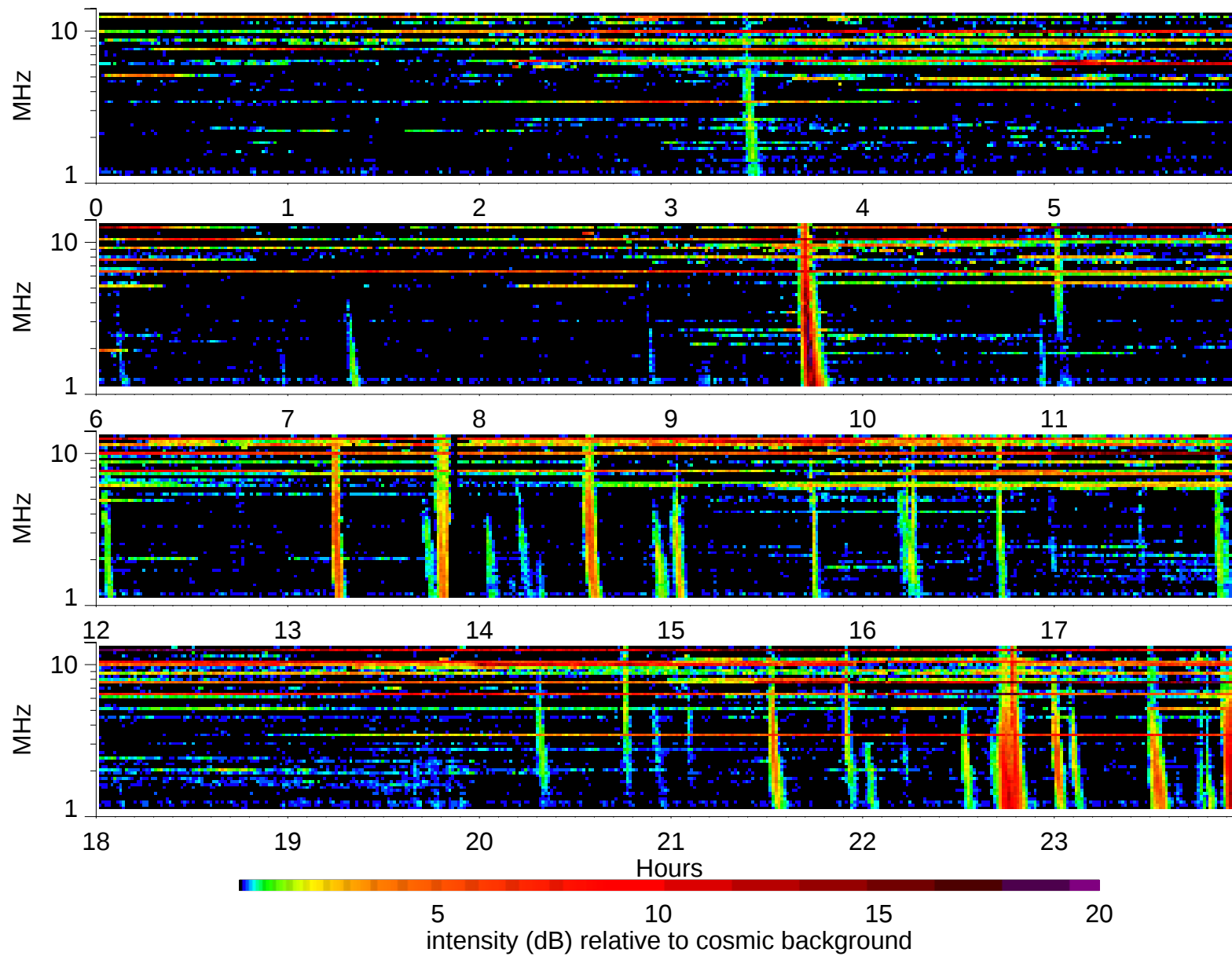
Wind Waves RAD2 receiver: 1999/3/10
